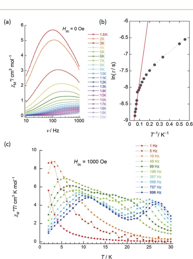
Fig. 4 Frequency ( \nu ) and temperature ( T ) dependence of the ac magnetic susceptibility ( \chi_M'' : out-of-phase) of 2 (SAP–SAP*). The measurements were performed in a 3 Oe ac magnetic field at the indicated \nu . (a) \nu dependence of \chi_M'' measured between 1.8 and 20 K in an H_{\text{dc}} of zero. The solid lines are guides for eyes. (b) Arrhenius plots for 2 in an H_{\text{dc}} of zero. Solid lines were fitted by using the Arrhenius equation (see main text). (c) \nu dependence of \chi_M''T versus T at H_{\text{dc}} of 1000 Oe. The solid lines are guides for eyes.
