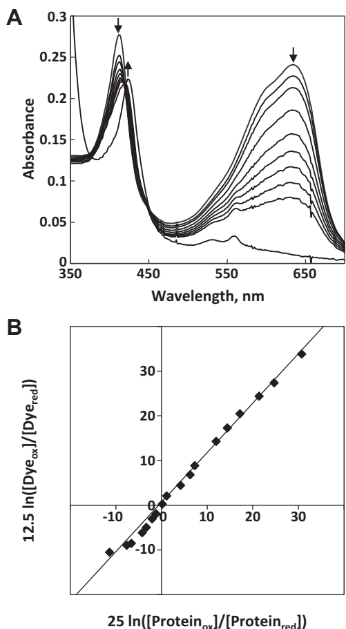
Fig. 1. (A) Spectroscopic changes observed during the determination of the \text{Fe}^{3+/2+} reduction potential of the PAS-A domain of hNPAS2 using the dye Nile blue (25.0 °C, pH 7.0). Arrows indicate direction of absorbance changes. (B) The corresponding Nernst plot.
