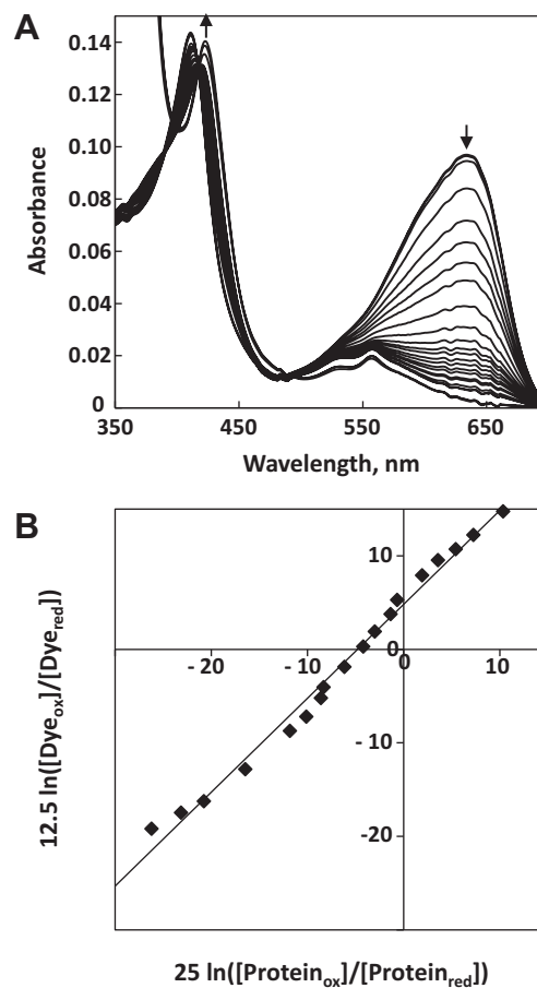
Fig. 2. (A) Spectroscopic changes observed during the determination of the \text{Fe}^{3+/2+} reduction potential of the PAS-A domain of hCLOCK using the dye Nile blue (25.0 °C, pH 7.0). Arrows indicate direction of absorbance changes. (B) The corresponding Nernst plot.
