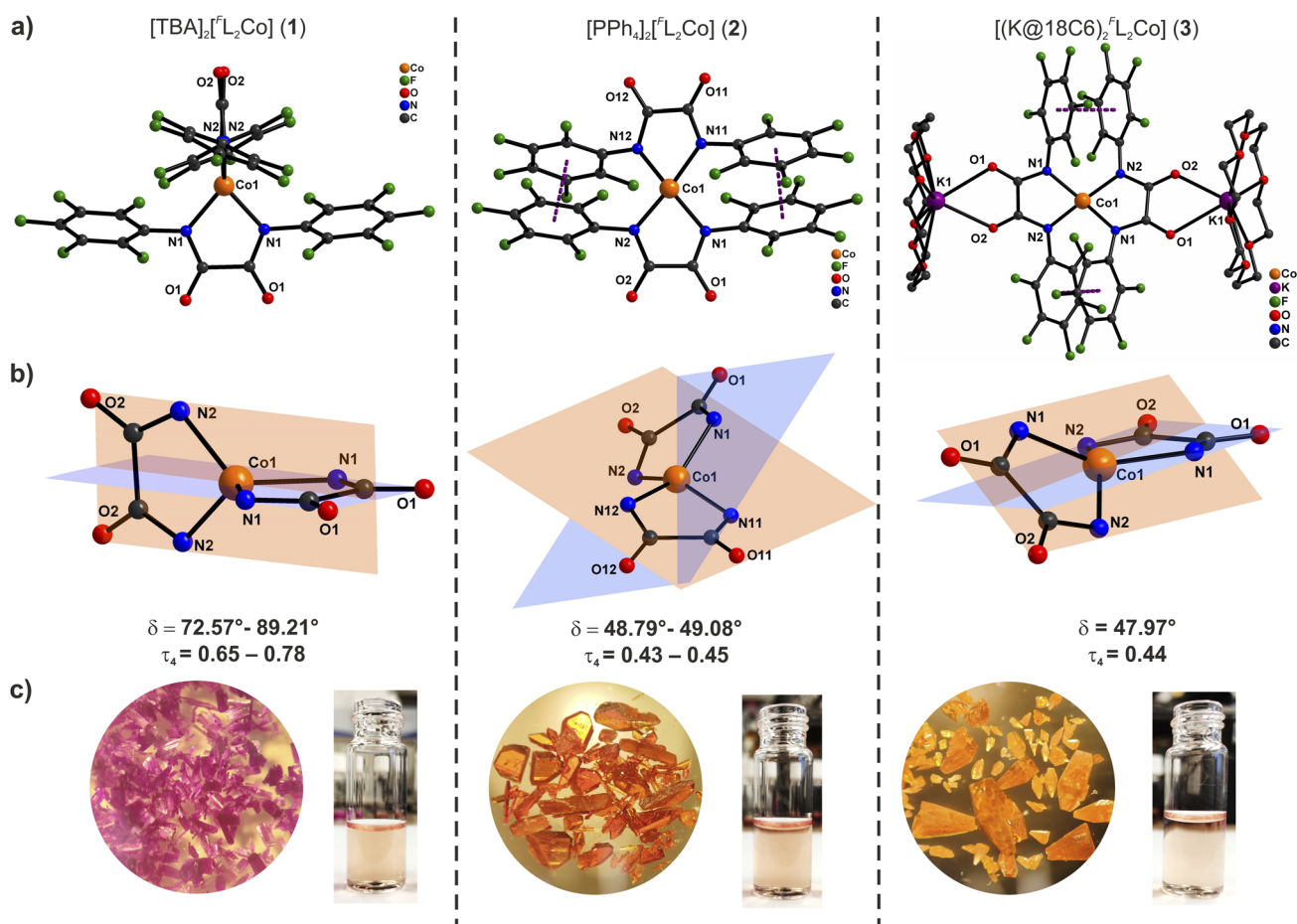
Fig. 1 (a) Molecular structures of the anions of 1 (left) and 2 (middle), and 3 (right); cations have been omitted for clarity in case of 1 and 2 . (b) Core structures of 1–3 showing the two intersecting N–Co–N chelate planes. (c) Complexes 1–3 in the solid state and DMF solution.
