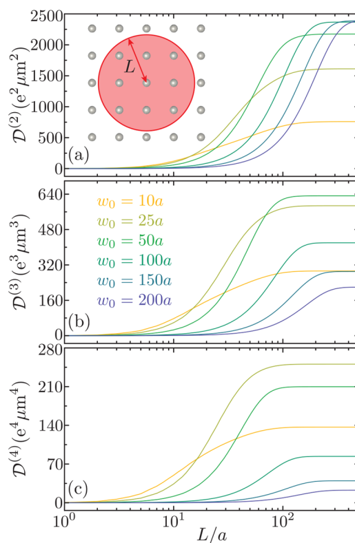
Figure 4. (a–c) Value of \mathcal{D}^{(n)} , defined in eq 5, as a function of L for n = 2 (a), 3 (b), and 4 (c). All calculations are performed for an array with a = 500 nm and D = 100 nm and different values of w_0 , as indicated by the legend.
