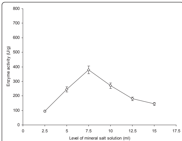
Figure 2 Effect of different levels of mineral salt solution (pH 5.5) as initial moisture content on AXE production from P. notatum NRRL-1249. Wheat bran (10 g) was used as a basal substrate and incubated at 30°C for 48 h. Y-bars show \pm sd among the triplicates.
