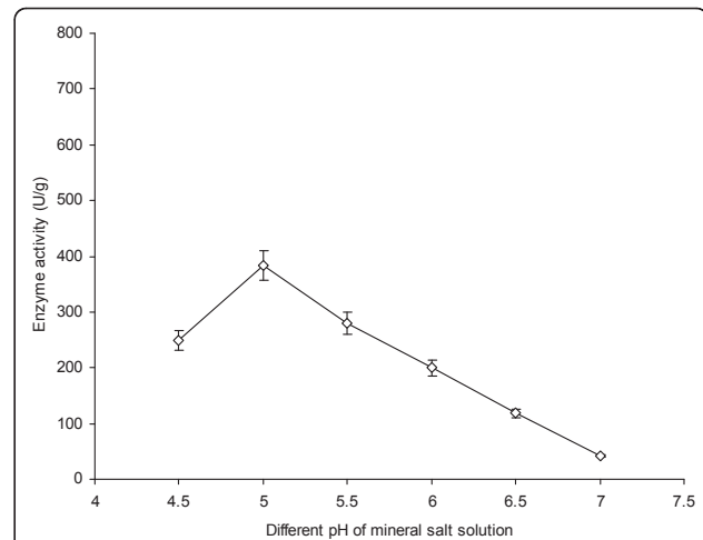
Figure 3 Effect of different pH of mineral salt solution on AXE production from P. notatum NRRL-1249. Wheat bran (10 g) was used as a basal substrate and moistened with MSS at a ratio of 1:0.75. The flasks were incubated at 30°C for 48 h. Y-bars show \pm sd among the triplicates.
