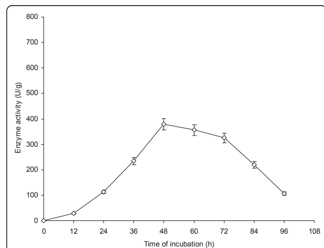
Figure 4 Time of incubation for AXE production from P. notatum NRRL-1249. Wheat bran (10 g) was used as a basal substrate and moistened with MSS (pH 5) at a ratio of 1:0.75. The flasks were incubated at 30°C. Y-bars show \pm sd among the triplicates.
