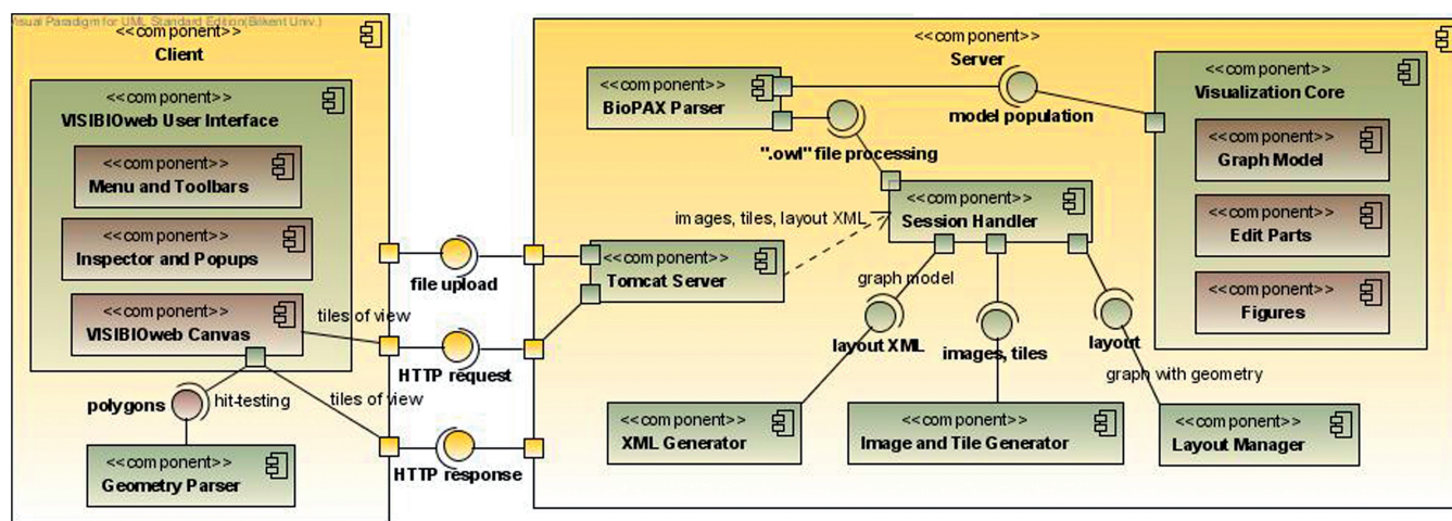
Figure 1. High-level architecture of VISIBIOweb depicted with a UML component diagram.
