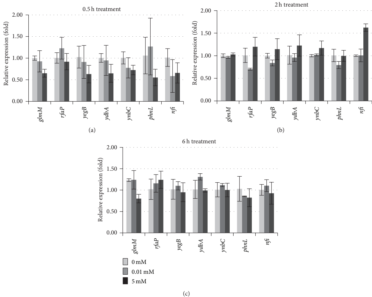
FIGURE 5: Transcript levels of seven selenite-responsive candidate genes quantified by qRT-PCR. The RNA samples were isolated from bacteria cells grown under 0, 0.01, or 5 mM \text{Na}_2\text{SeO}_3 treatment for (a) 0.5, (b) 2, or (c) 6 h. Data shown are fold changes calculated as transcript levels of selenite treated samples compared to untreated (defined as 1). Data represent an average of three biological replicates \pm SD. Each replicate was assayed in triplicate.
