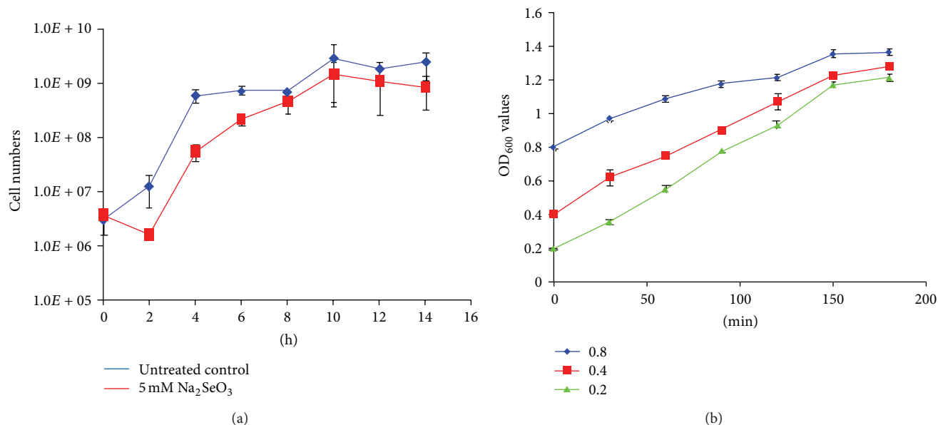
FIGURE 3: The growth curve of bacterial cells. The growth curve of cells cultured with or without 5 mM Na 2 SeO 3 (a). The growth curve of cells cultured with initial culture concentrations of OD 600 values of 0.2, 0.4, and 0.8 (b). Each experiment was performed with three biological replicates and each treatment was assayed in triplicate. Data plotted was the average \pm SD.
