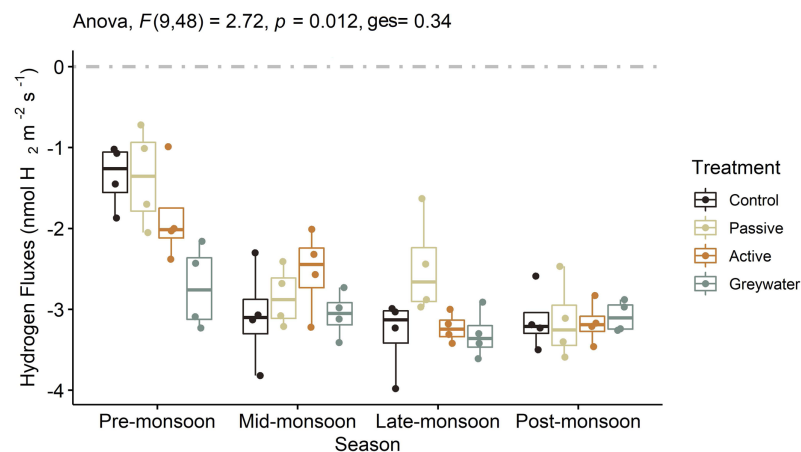
Figure 2 The effects of green infrastructure management and time during the monsoon season on soil hydrogen fluxes (nmol H 2 m -2 s -1 ). Boxplots displayed with point distributions for each batch within a treatment. The center line represents the median, and the lower and upper lines correspond to the first and third quartiles (25% and 75% quartiles). Whiskers correspond to the 95% confidence intervals. The two-way ANOVA presented F statistic, p -value and generalized eta squared ( ges ). The grey dashed line at 0 on the y -axis represents the transition between soil uptake (negative values) and emission into the atmosphere (positive values).
