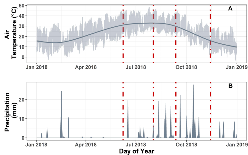
Figure 1 Meteorological data measured hourly on site. (A) Site level air temperature (°C) measured at 3 m aboveground. Light grey represents the hourly temperature. Dark grey line represents the smooth fit function from a generalized additive model estimation of air temperature. (B) Daily cumulative sum of precipitation (mm) at the site. Dashed red lines represent the static chamber hydrogen sampling dates.
