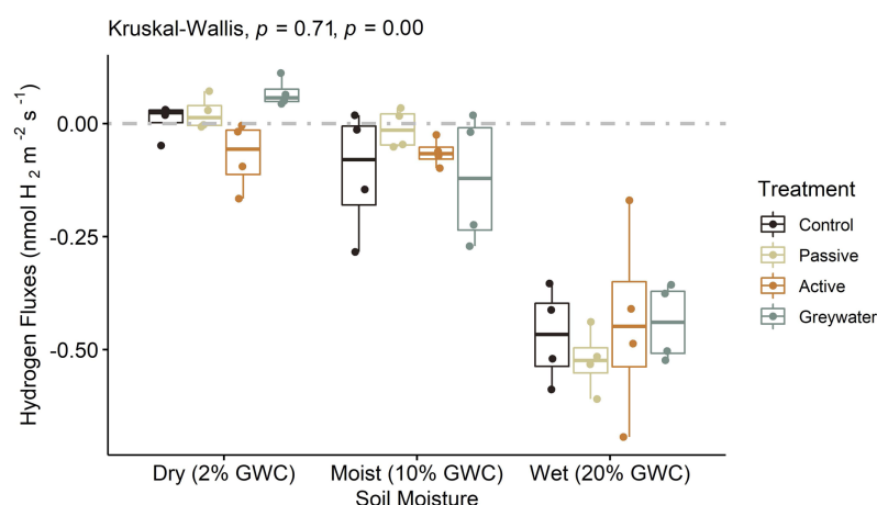
Figure 3 Microcosms assessing the effects of green infrastructure management and soil moisture on hydrogen fluxes ( \text{nmol H}_2 \text{ m}^{-2} \text{ s}^{-1} ). Boxplots displayed with point distributions for each batch within a treatment. The center line represents the median, and the lower and upper lines correspond to the first and third quartiles (25% and 75% quartiles). Whiskers correspond to the 95% confidence intervals. The one-way nonparametric Kruskal-Wallis ANOVA was performed independently for both treatment and moisture level on \text{H}_2 . Corresponding p -values are recorded with treatment first and moisture level second. The grey dashed line at 0 on the y-axis represents the transition between soil uptake (negative values) and emission into the atmosphere (positive values).
