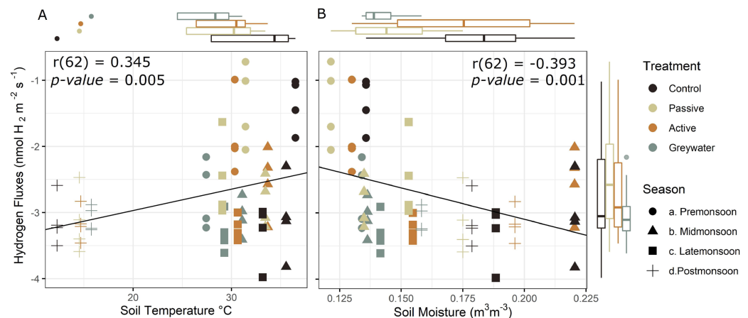
Figure 4 Effect of selected environmental drivers during in situ measurements of soil hydrogen fluxes (nmol H 2 m -2 s -1 ). (A) Positive correlation of hydrogen fluxes and soil temperature °C shows H 2 uptake into the soil is greater at lower temperature, and (B) negative correlation between hydrogen fluxes and soil moisture indicates that H 2 uptake increases with increased moisture. Boxplots display the median, 25th and 75th interquartile range, and whiskers show 1.5 times the interquartile for soil temperature (top left), soil moisture (top right), and soil hydrogen fluxes (right side) averaged during the in situ sampling period. Negative H 2 fluxes indicate uptake from the atmosphere into the soil.
