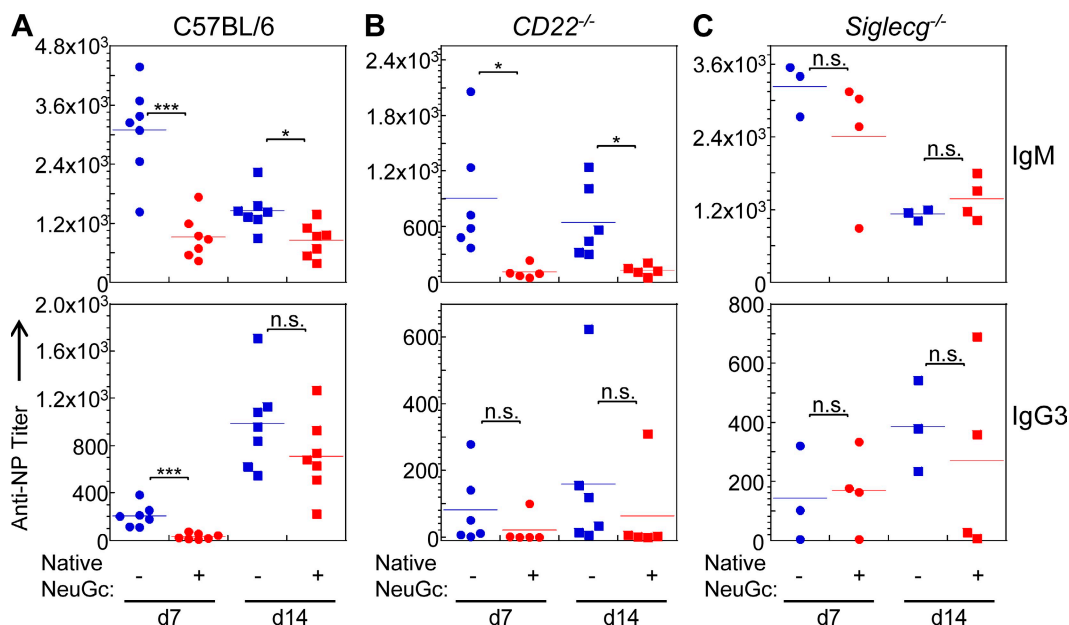
Figure 3. Serum anti-NP responses to unsialylated (–; NP-PA) or natively sialylated (+; NP-PA-NeuGc) compounds. (A–C) Responses of (A) wild-type, (B) CD22 -/- , and (C) Siglecg -/- mice. Anti-NP titers were assessed on days 7 and 14 as indicated. (top) IgM anti-NP titers; (bottom) IgG3 anti-NP titers. Each point represents the response of an individual mouse of the indicated genotype. Results shown are representative of at least two independent experiments. Horizontal bars represent means. *, P < 0.05 ; and ***, P < 0.005 using the two-tailed Student's t test. n.s., not significant.
