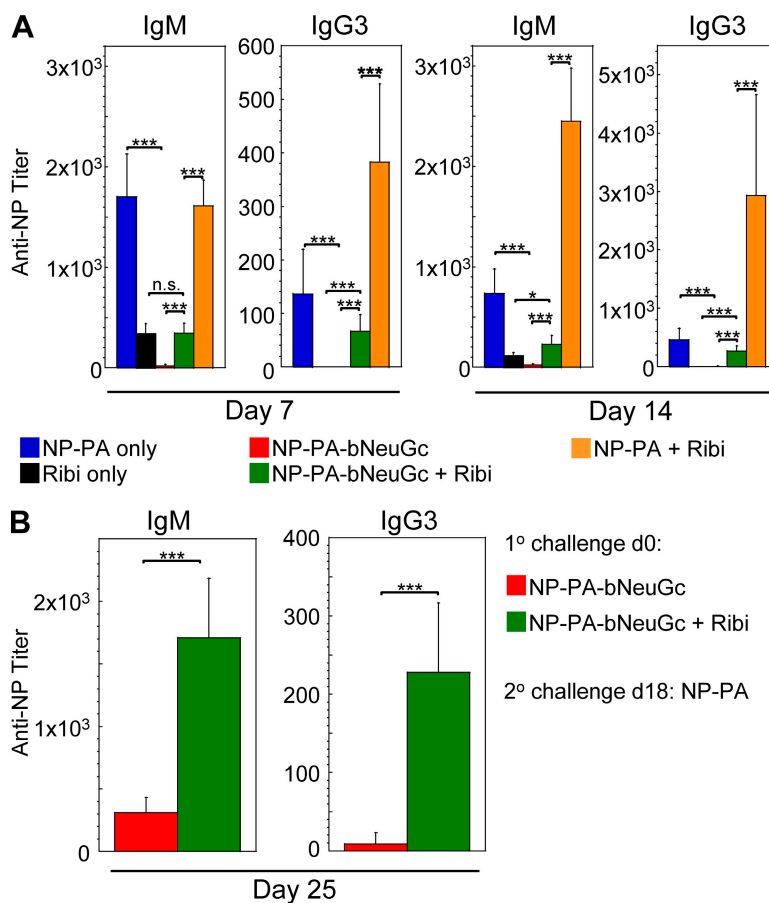
Figure 5. Effect of Ribl coadministration on tolerance induction and response to sialylated and unsialylated antigens. (A) Mice received the indicated conjugates in the presence or absence of Ribl; serum IgM and IgG3 anti-NP levels were measured on days 7 and 14. (B) Mice were treated with the tolerogenic compound NP-PA-bNeuGc with or without Ribl on day 0, and were rechallenged on day 18 with NP-PA. Shown are serum anti-NP titers monitored on day 25. Results are representative of three experiments. For all experimental groups, eight mice were analyzed. Shown are means + SD. All statistical tests given used the two-tailed Student's t test. *, P < 0.05 ; ***, P < 0.005 . n.s., not significant.
