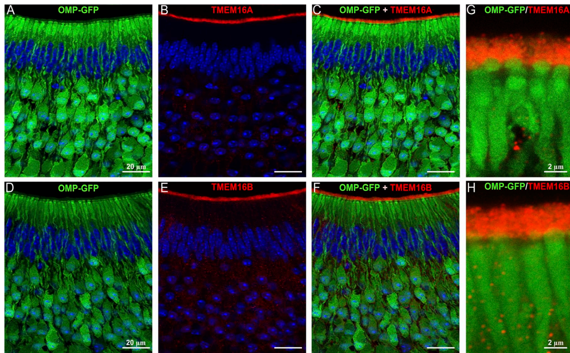
Figure 7. TMEM16A and TMEM16B are expressed at the apical surface of the vomeronasal epithelium. (A–H) Immunostaining of sections of VNO from an OMP-GFP mouse. (A and D) Endogenous GFP fluorescence of mature vomeronasal sensory neurons. TMEM16A (B) and TMEM16B (E) are expressed at the luminal surface of the vomeronasal sensory epithelium. (G and H) High magnification image of the apical portion of the VNO showing that TMEM16A and TMEM16B are expressed at the apical surface. Cell nuclei were stained by DAPI (blue). Bars: (A–F) 20 \mu m ; (G and H) 2 \mu m .
