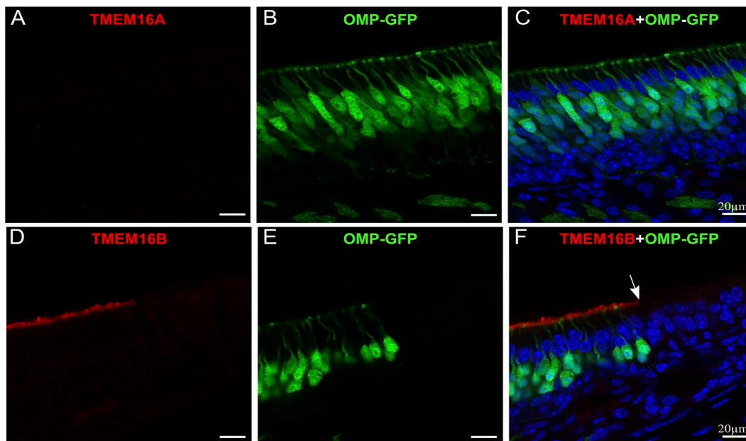
Figure 6. TMEM16A and TMEM16B immunoreactivity in the olfactory epithelium. (A–C) Confocal images of coronal sections of the olfactory epithelium from an OMP-GFP mouse showing the absence of TMEM16A immunoreactivity. (D–F) Confocal images of the transition region between the olfactory and the respiratory epithelium (absence of OMP-GFP-expressing neurons). The arrow indicates the transition between the two epithelia. TMEM16B is expressed at the apical surface of the olfactory but not of the respiratory epithelium. Cell nuclei were stained by DAPI (blue). Bars, 20 μm.
