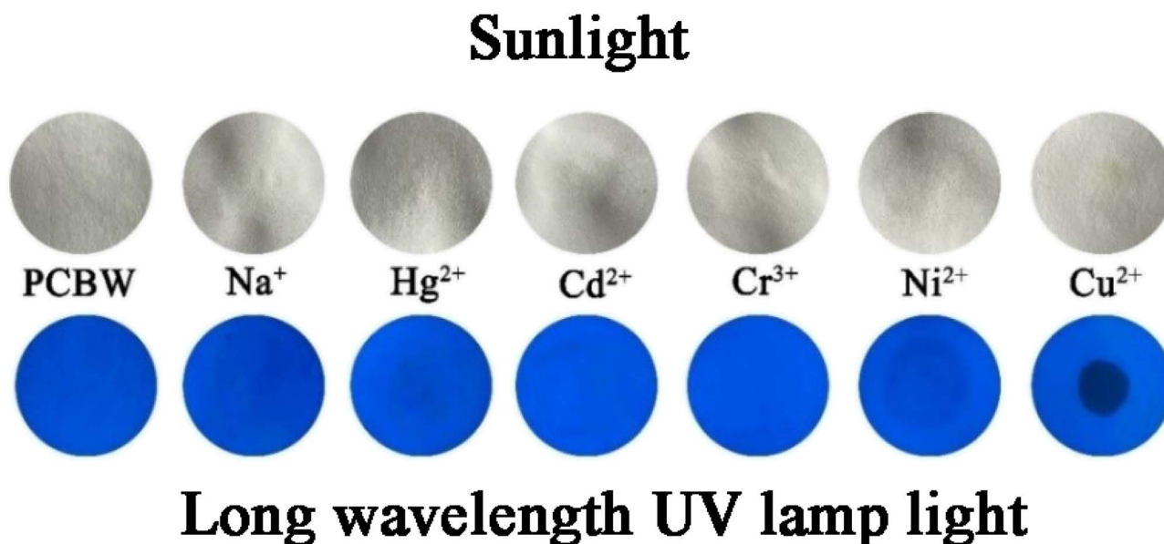
Fig. 11 The photographs of PCBW-based test strips upon addition of Na + , Hg 2+ , Cd 2+ , Cr 3+ , Ni 2+ , and Cu 2+ under sunlight and long wavelength UV lamp light.
