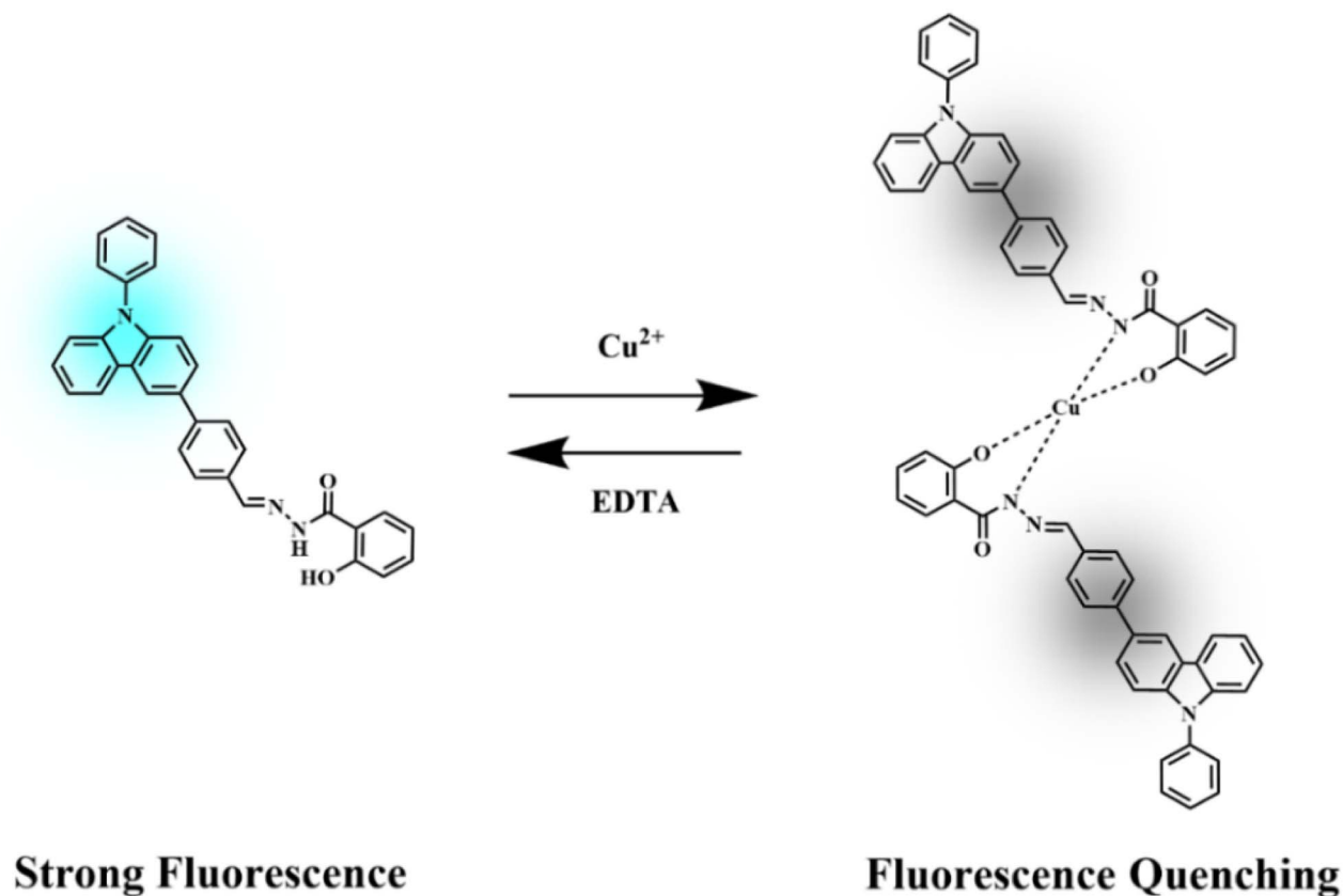
Scheme 2 A proposed binding mode between PCBW and \text{Cu}^{2+} .
