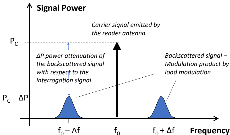
Figure 19. Load modulation creates two sidebands around the transmission frequency f_0 of the reader. The actual information is carried in the sidebands of the two subcarrier sidebands, which are themselves created by the modulation of the subcarrier.
