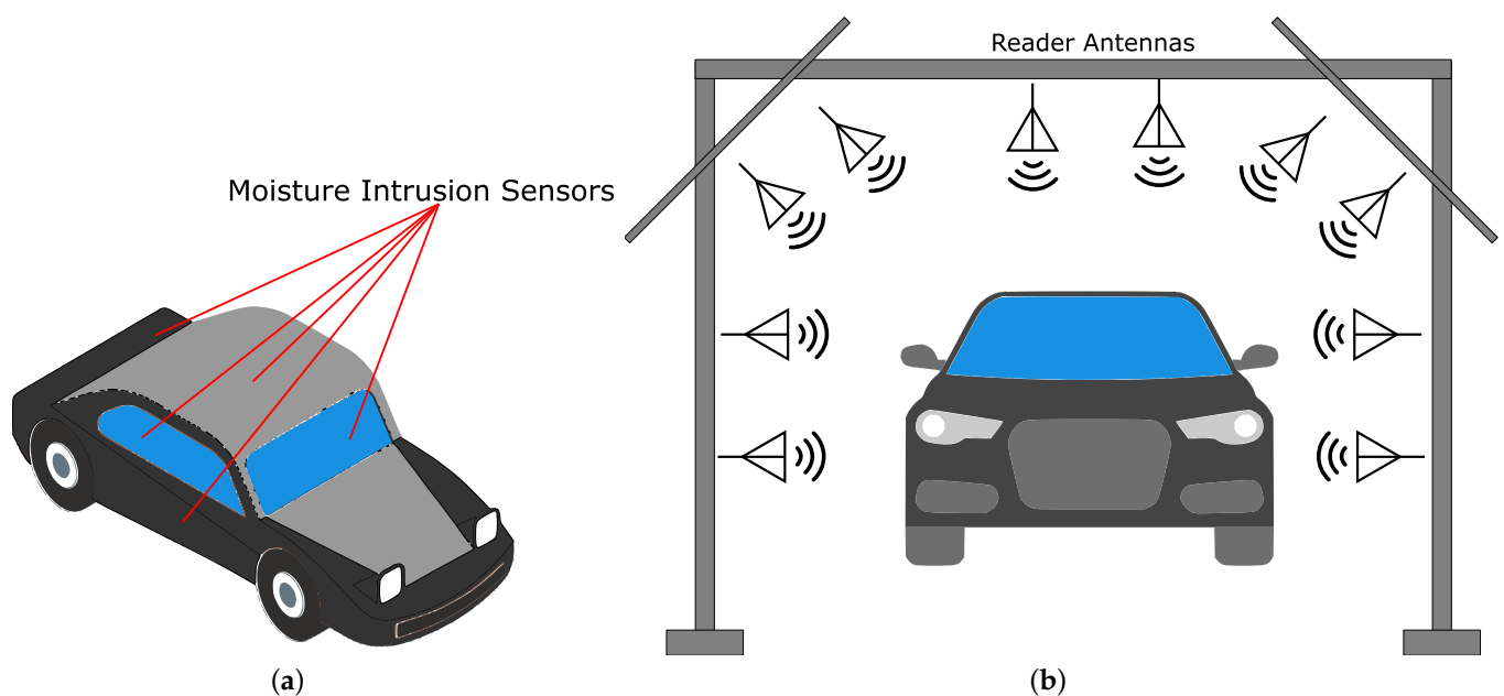
Figure 18. RFID sensors for the moisture intrusion detection system: (a) Moisture sensors placed directly on the vehicles' metal chassis; (b) Interrogation setup.
