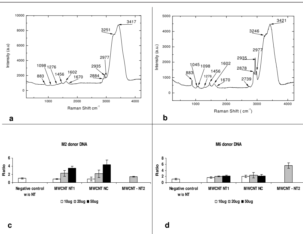
Figure 4 shows signal of DNA in the region until 2000\text{ cm}^{-1} . DNA consist of three groups: phosphates, deoxyribose and four bases such as A (adenine), T (thymine), C (cytosine) and G (guanine). In our work, the bands could be assigned to 883/1098/1045\text{ cm}^{-1} - O-P-O backbone; 1276\text{ cm}^{-1} - C (cytosine); 1456\text{ cm}^{-1} - A (adenine); 1602\text{ cm}^{-1} - guanine (G) and 1670\text{ cm}^{-1} - T (thymine). The bands of DNA donor M2 (a) and M6 (b) are in accordance with some authors [21,22]. The bands 2739\text{-}3421\text{ cm}^{-1} are not assigned to DNA, it is assigned to the quartz substrate. In (c) and (d) it shows the action of the MWCNT under Neisseria meningitidis strain C2135 using as donor DNA the M2 (c) and M6 (d).
