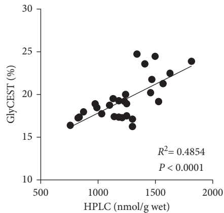
FIGURE 5: Correlation between HPLC and GlyCEST measurements. GlyCEST (%) is significantly correlated with the glycine concentration measured by HPLC.
