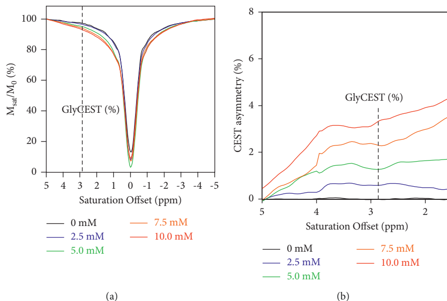
FIGURE 1: GlyCEST effects. (a) z-spectra of a phantom containing different glycine concentrations (pH 7.0). (b) CEST asymmetry at various saturation offsets for different glycine concentrations. The same computation was used to determine GlyCEST (%).
