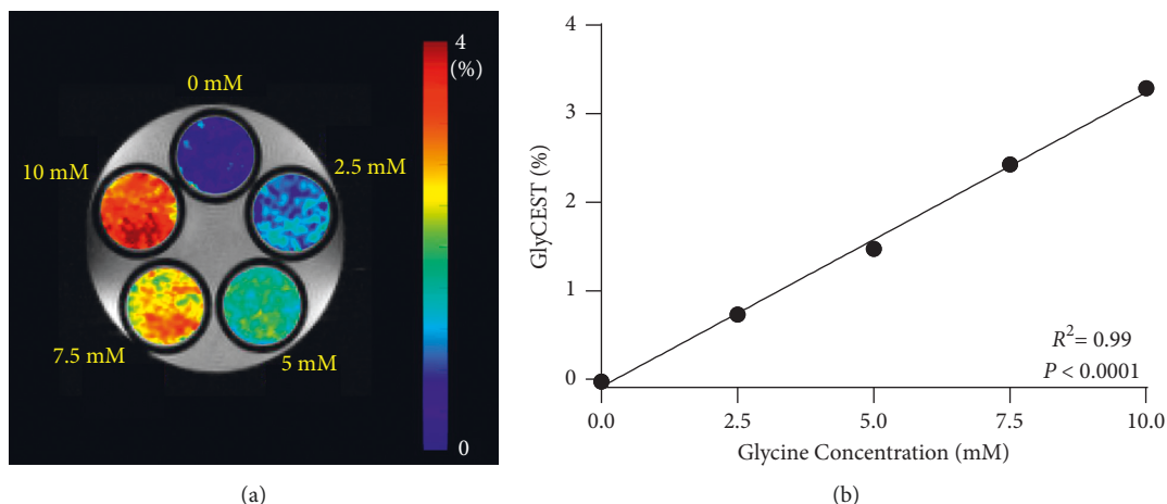
FIGURE 2: (a) GlyCEST map of a phantom. (b) Significant linear correlation between GlyCEST (%) and glycine concentration.
