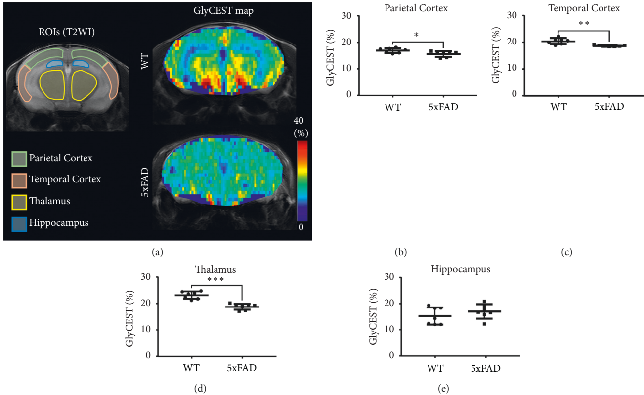
FIGURE 4: GlyCEST effects in WT ( n = 7 ) and 5xFAD ( n = 7 ) mice. (a) T2WI ROIs in a coronal brain slice (left panel) and the corresponding GlyCEST maps (right panel). (b–e) GlyCEST (%) of the parietal and temporal cortex, thalamus, and hippocampus. Data were analyzed using the unpaired t -test. * P < 0.05 , ** P < 0.005 , and *** P < 0.0001 .
