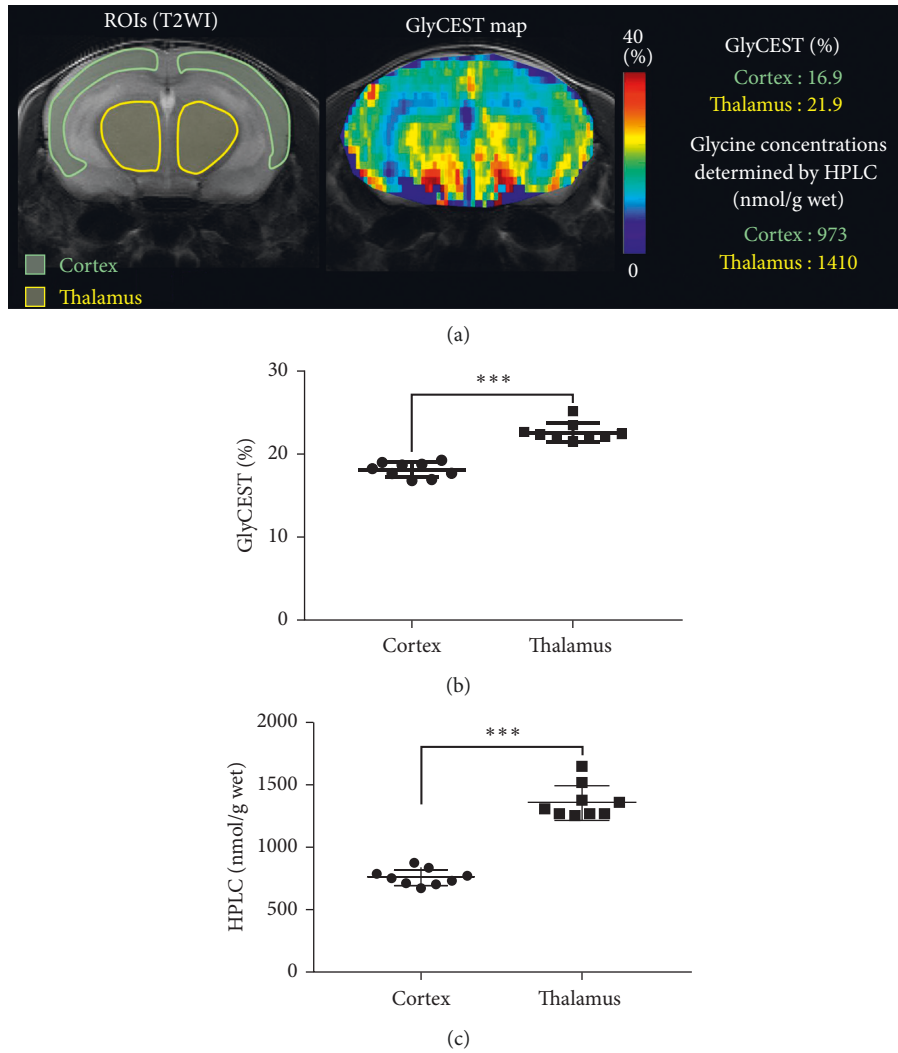
FIGURE 3: GlyCEST effects and glycine concentrations in C57BL/6 wild-type (WT) mice ( n=9 ). (a) T2-weighted spin-echo image (T2WI) showing regions of interest (ROIs) in a coronal brain slice (left panel) and the corresponding GlyCEST map (center panel). The corresponding GlyCEST (%) and glycine concentrations detected by high-performance liquid chromatography (HPLC) analysis in the cortex and thalamus are also shown (right panel). (b) GlyCEST (%) in the cortex and thalamus measured in T2WI-defined ROIs. (c) Glycine concentrations in the cortex and thalamus detected by HPLC. In both GlyCEST and HPLC measurements, the glycine concentration in the thalamus is higher than that in the cortex. Data were analyzed using the paired t -test (***) P < 0.0001 .
