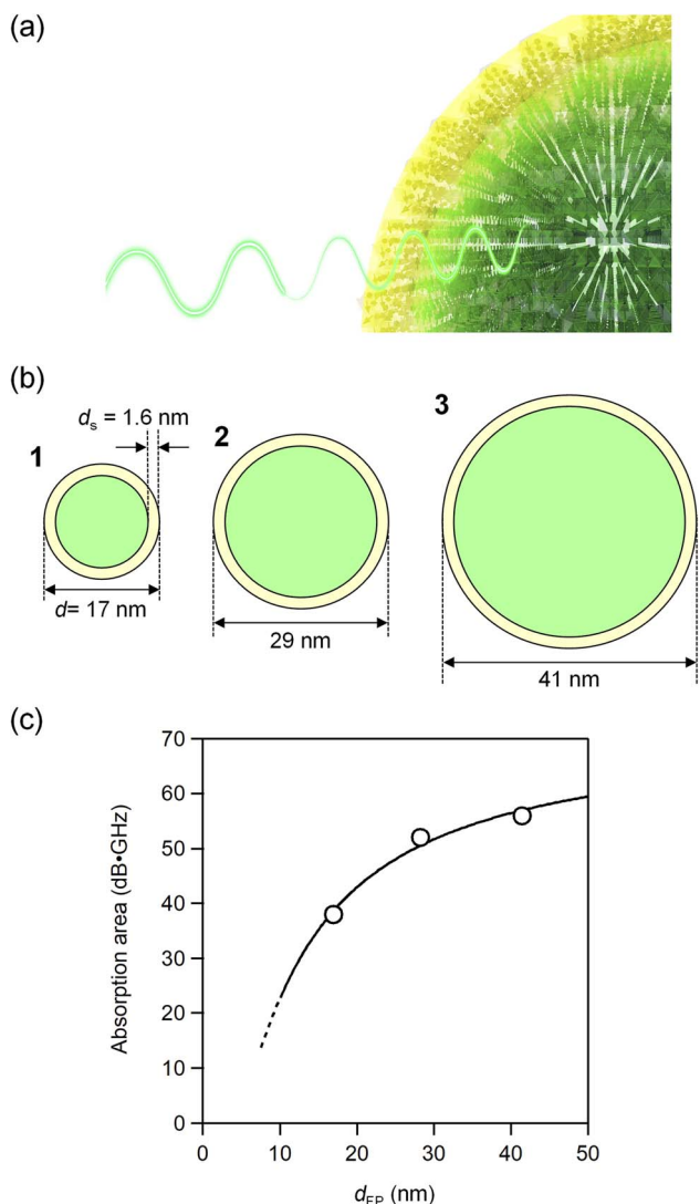
Fig. 4 (a) Schematic illustration of millimeter wave absorption. The core (green) absorbs millimeter waves but the surface (yellow) does not. (b) Schematic illustration of the nanoparticles of 1–3 showing the thickness from the surface d_s . (c) Absorption peak area versus the particle size (open circles) and the fitted line by eqn (1) (solid line).
