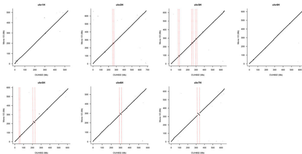
Figure 2 Alignment of pseudomolecules of “OUH602” to “Morex” V3 by a single chromosome. Areas between dotted red lines show inversions.
