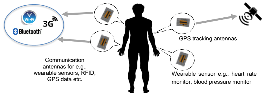
Figure 1. Examples of wearable antennas integrated with wearable electronic devices for many applications. Through wearable technology, various Internet of Things (IoT) applications can be supported such as healthcare monitoring via wearable sensors, human tracking through body-centric radio-frequency identification (RFID), sportsmen or patient tracking via a wearable global positioning system (GPS) receiver and many more.
