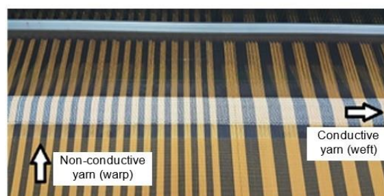
Figure 2. Warp and weft of the manufactured electro-textile fabric. The conducting part was made from a mixture of copper and polyester threads, with the weight ratio of 83% and 17% for copper and polyester, respectively.
