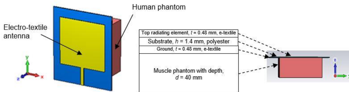
Figure 7. Configuration for on-body condition analysis (Case B). During simulation, the antenna is attached to the human phantom with various dielectric constant, \epsilon_r and conductivity, \sigma to represent the exact properties of human body fat, muscle and blood.
