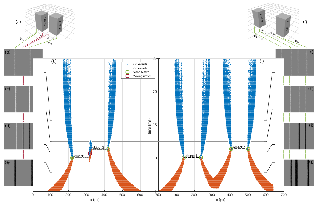
Figure 7. Highlighting of the wrong depth measurements for two closely spaced edges. The two central plots show events in the x-time plane, smashing the y-dimension. Events are color coded with their polarity (red for OFF events, blue for ON events). The right one is a valid case, with no overlap. The left one contains an overlap in the event stream, leading to wrong depth deductions in this case. 4 snapshots of events are presented for every case.
