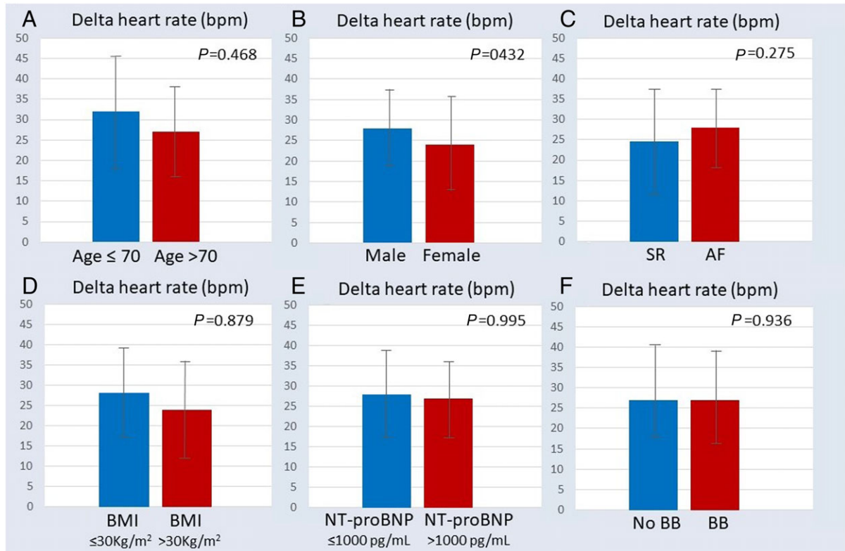
Figure 1 Delta heart rate across subgroups of age, gender, type of rhythm, body mass index, NT-pro-BNP, and beta-blocker treatment. AF, atrial fibrillation; BB, beta-blocker treatment; BMI, body mass index; NT-pro-BNP, N-terminal pro-BNP; SR, sinus rhythm.
