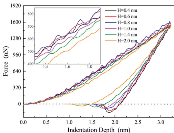
Fig. 2 Force-indentation depth curve under different SiO 2 film thickness ( H ).
