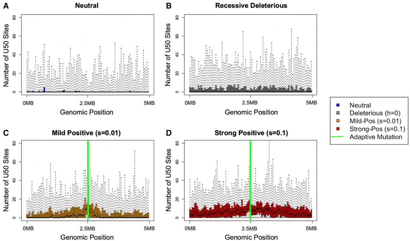
Figure 3 U50 statistics under Model_0. (A–D) show the distributions of U50 statistic in 50-kb windows across the 5-Mb region on Chr11. U50 is the number of sites with an archaic allele that has frequency >50% in the recipient population. For each 50-kb window (the x-axis), we plot the interquartile distributions of U50 over 200 simulation replicates in boxes, with whiskers extending to all data points. Mutations are (A) neutral, (B) recessive and deleterious with selection effects drawn from a gamma DFE, (C) same as (B) with a single mildly beneficial ( s = 0.01 ) mutation, and (D) same as (B) with a single highly beneficial ( s = 0.1 ) mutation. Recombination was simulated at a uniform rate of 1e-9 per site. The adaptive mutations in (C and D) are placed in a window in the middle of the region (2.5 Mb), indicated by the green solid line. We simulated under the demography described by Model_0 (see Figure 2).
