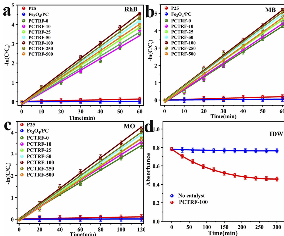
Fig. 12 Reaction kinetics curves with error bars for the photocatalytic degradation of: (a) RhB, (b) MB, and (c) MO using P25, \text{Fe}_3\text{O}_4/\text{PC} , and Ru-TiO 2 /PC/ \text{Fe}_3\text{O}_4 series samples. (d) Non-linear kinetics curve for the photocatalytic degradation of actual dye wastewater using the PCTRF-100 sample.
