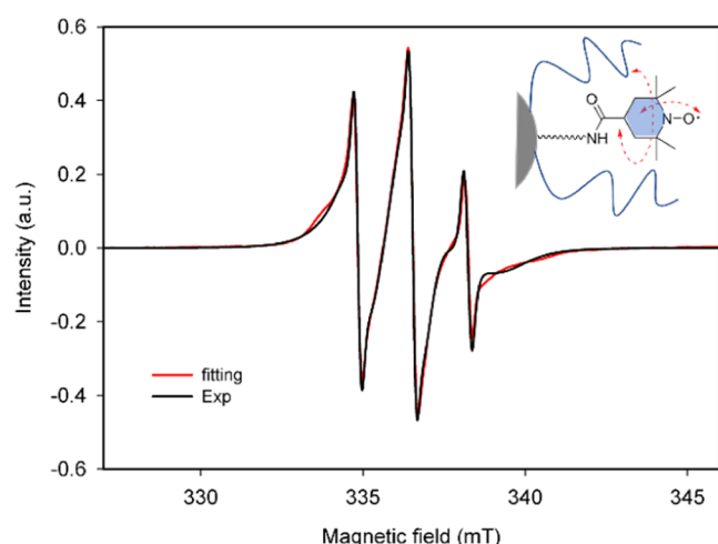
Figure 3. Experimental and simulated EPR spectrum of PluS-NO ( 2 \times 10^{-5} M in water).
