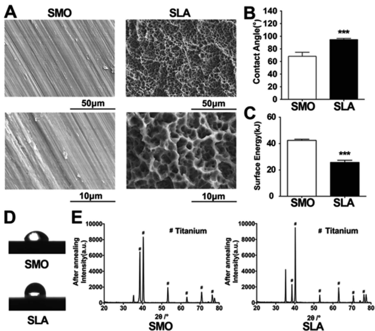
Fig. 1 Physicochemical properties of prepared SLA and SMO surfaces. (A) Scanning electron microscopy observation of smooth polished (SMO) titanium, and sandblasted and acid-etched (SLA) titanium surface samples at two magnifications. (B) Contact angle (CA) in distilled water. (C) Surface energy in water. (D) Images of the CA measurement of distilled water. (E) X-ray diffraction patterns of SMO and SLA titanium samples after heat treatment. Data are presented as the mean \pm s.d. ( n = 6 ). *** p < 0.001 .
