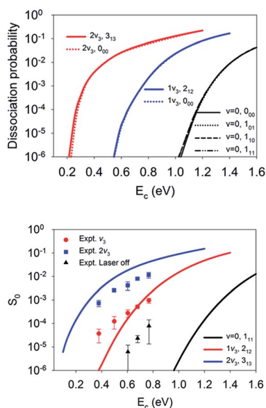
Fig. 7 The upper panel displays site-averaged dissociation probabilities as a function of collision energy of the M -averaged D_2O(v=0, 0_{00}, 1_{01}, 1_{10}, 1_{11}) , D_2O(1\nu_3, 2_{12}) , and D_2O(2\nu_3, 3_{13}) states. The lower panel shows a comparison of sticking probabilities with the lattice effects corrected of the D_2O(v=0, 1_{11}) , D_2O(1\nu_3, 2_{12}) , and D_2O(2\nu_3, 3_{13}) states and available experimental data. 65
