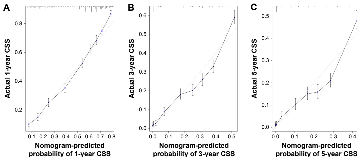
Figure 4 External calibration plot. Note: (A) 1-year, (B) 3-year, and (C) 5-year CSS nomogram calibration curves. Abbreviation: CSS, cancer-specific survival.
