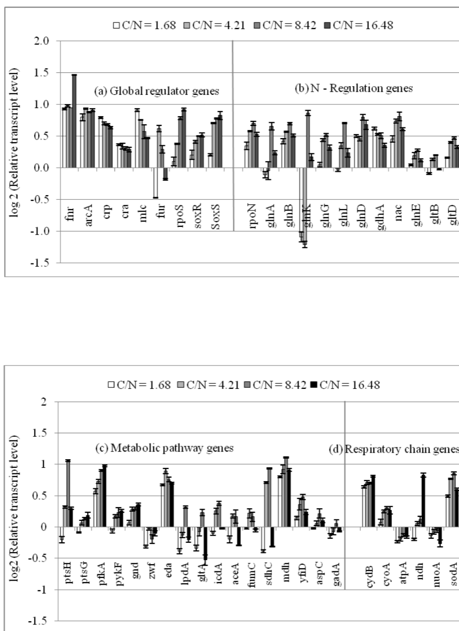
Figure 3 Comparison of the transcriptional mRNA levels of the wild type E.coli genes cultivated at 100% (C/N = 1.68), 40% (C/N = 4.21), 20% (C/N = 8.42) and 10% (C/N = 16.48) N- concentration: (a) global regulatory, (b) N- regulatory, (c) metabolic pathway, (d) respiratory chain.
