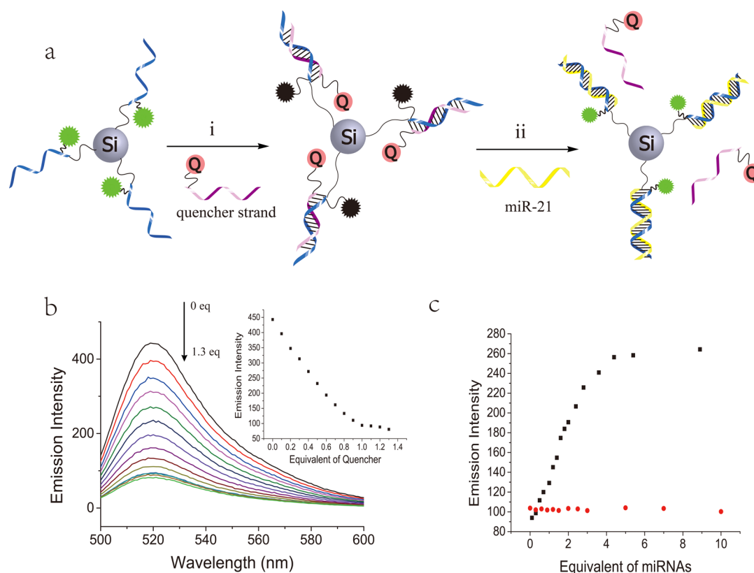
Figure 3. (a) Schematic illustrating the use of SiNP ODN conjugates to detect miR-21. (i) The quencher strand hybridizes with the SiNP ODN conjugate leading to a fluorescence OFF state. (ii) miR-21 binds to the SiNP ODN conjugate leading to displacement of the quencher strand, resulting in a fluorescence ON state. (b) Quenching of SiNP ODN conjugate upon addition of increasing equivalents of the quencher ODN. Inset: Fluorescence quenching profile with increasing equiv of quencher ODN, followed at 520 nm. (c) Fluorescence enhancement profile in the presence of increasing amounts of miR-21 (black) and control miR-155 (red). Note: For these fluorescence experiments the fluorescein unit on the SiNP ODN conjugates were excited at 490 nm and the concentration of conjugated ODNs was 500 nM.
