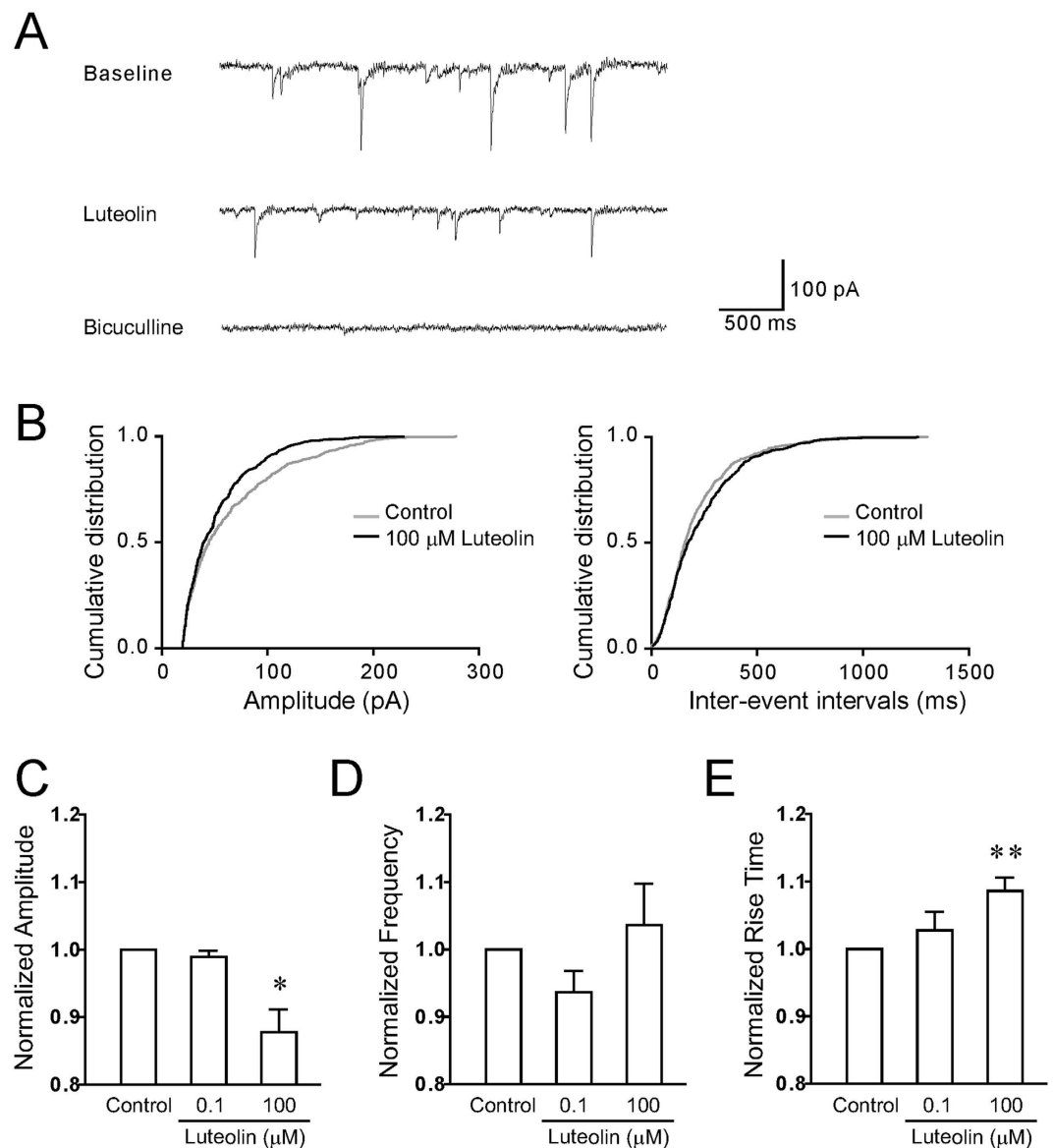
Figure 5. The effect of luteolin on mIPSCs in hippocampal slices. (A) Representative traces showed mIPSCs recorded before (top trace) or after 100 \mu\text{M} of luteolin treatment (middle trace) in a hippocampal CA1 pyramidal neuron. 10 \mu\text{M} of bicuculline was applied at the end of the experiment to eliminate mIPSCs (bottom trace). (B) Cumulative probability plots of mIPSC amplitudes (left) and inter-event intervals (right) from the recorded neuron shown in (A). (C–E) Summary of changes in mean mIPSC amplitudes (C), mean frequencies (D), and mean rise time (E) after 0.1 ( n=7 ) or 100 \mu\text{M} ( n=9 ) luteolin treatments. All data points and bars represent mean values \pm s.e.m. * P < 0.05 , ** P < 0.01 compared with control using one-way ANOVA.
