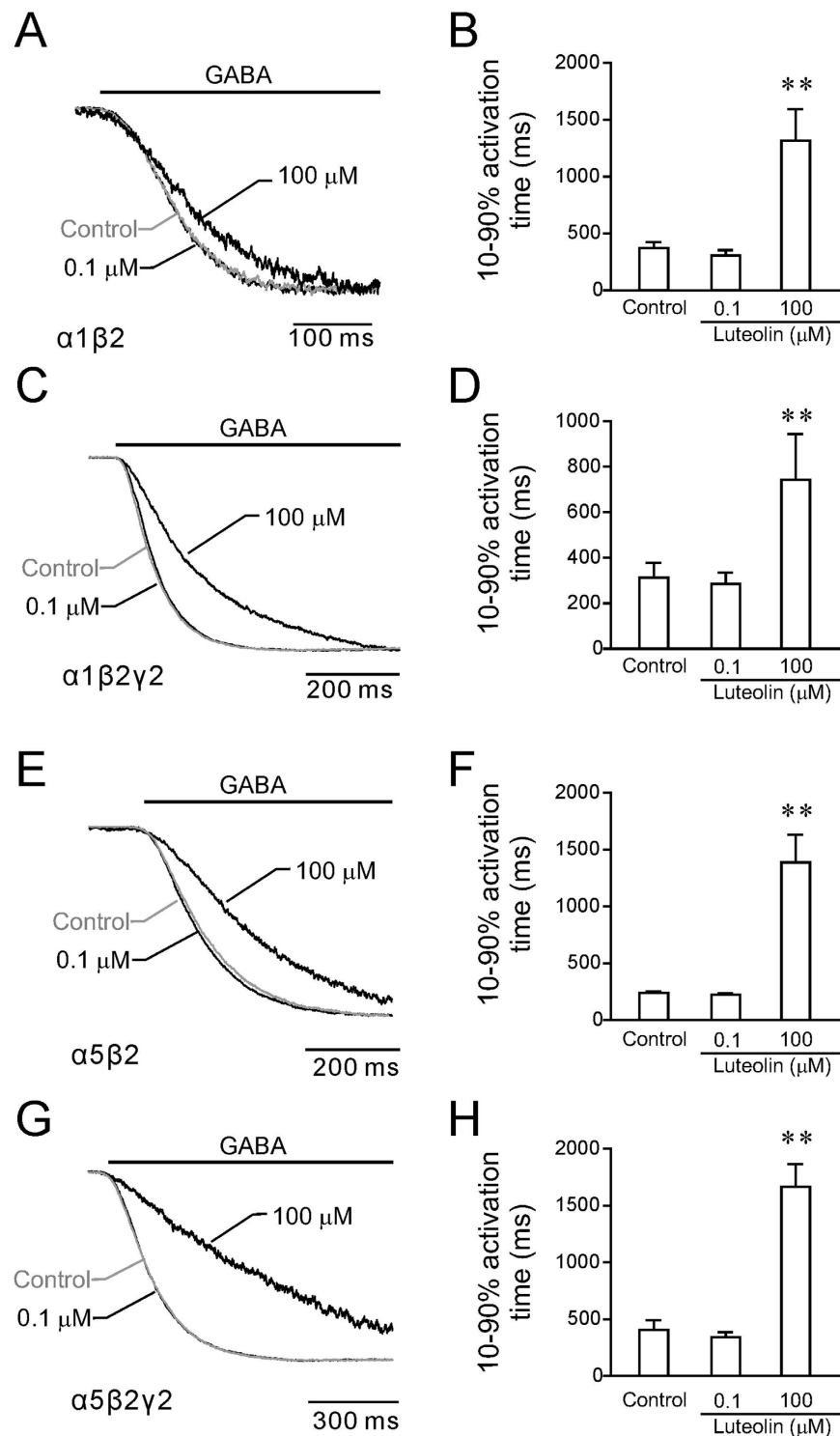
Figure 4. Luteolin slowed the activation of recombinant GABA A Rs. Representative current traces (superimposed and scaled) illustrating the effect of 0.1 and 100 \mu\text{M} of luteolin on current activation of \alpha 1\beta 2 (A), \alpha 1\beta 2\gamma 2 (C), \alpha 5\beta 2 (E), and \alpha 5\beta 2\gamma 2 receptors (G). The quantitative results summarized the 10–90% activation time calculated for control currents or after 0.1 and 100 \mu\text{M} of luteolin in \alpha 1\beta 2 (n = 15) (B), \alpha 1\beta 2\gamma 2 (n = 10) (D), \alpha 5\beta 2 (n = 10) (F), and \alpha 5\beta 2\gamma 2 receptors (n = 10). All data points and bars represent mean values \pm s.e.m. **P < 0.01 compared with control using one-way ANOVA.
