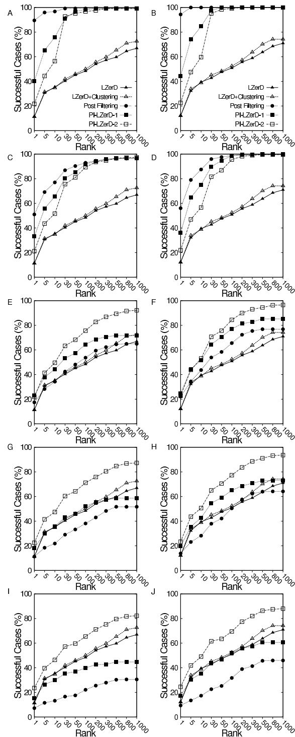
Figure 5 Docking prediction with simulated protein interface predictions. Four other methods are listed to compare with PI-LZeRD-2: the base LZeRD (LZeRD), LZeRD with clustering using ciRMSD (LZeRD+Clustering), LZeRD with one interaction of modified LZeRD (PI-LZeRD-1), and Simple residue filtering method (post-filtering). The x-axis indicates the ranks in logarithmic scale and the y-axis shows the percentage of cases where correct predictions are ranked equal or better than the corresponding ranks. Left panels, A, C, E, G, I , use the 2.5 Å as threshold for correct predictions, while right panels, B, D, F, H, J , use 4.0 Å as the cutoff for near hit predictions. A & B use the correct protein interface information; C/D use the simulated predictions with 5 residue shifts, E/F, G/H , and I/J use the simulated predictions with 10, 12, and 15 residue shifts, respectively.
