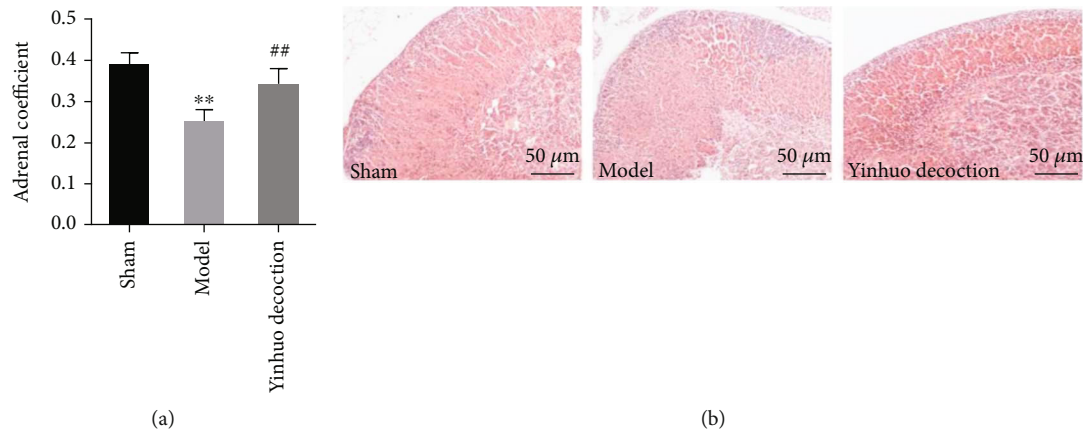
FIGURE 2: Yinhuo Decoction increased adrenal coefficient and relieved adrenal lesions in PMD model mice. (a) The adrenal coefficient in indicated groups and adrenal coefficient = adrenal gland weight (mg)/body weight (g) \times 100%. (b) H&E staining was used to evaluate the pathological changes of adrenal glands in each group. Magnification = 200x, scale = 50 \mu m; PMD: postmenopausal depression; H&E: hematoxylin and eosin staining; ** P < 0.01 indicated vs. Sham group; ## P < 0.01 indicated vs. Model group.
