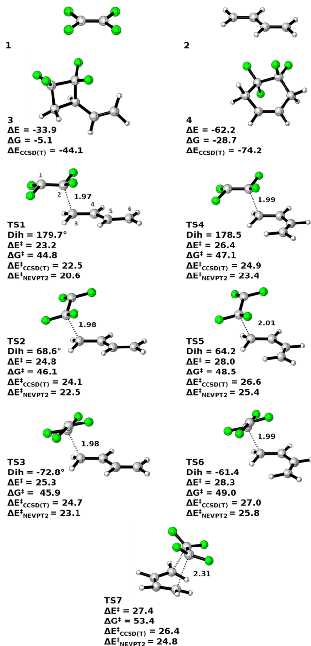
Figure 2. UB3LYP/6-311++G(d,p) optimized geometries and relative ΔE and ΔG 635K energies of diradical-forming transition states (TS1–TS6) and the Diels–Alder transition state, TS7. Values shown are the forming bond length (C2–C3, in Å) and dihedral (C1–C2–C3–C4, indicating anti, gauche +, and gauche –) angle about the forming bond. Energies are relative to reactants 1 and 2 and are in kcal/mol. DLPNO-UCCSD(T)/cc-pVTZ//UB3LYP/6-311++G(d,p) and in case of transition states NEVPT2/def2-TZVP//UB3LYP/6-311++G(d,p), single-point electronic energies are also given. Numbering of carbon atoms in TS and intermediates is demonstrated in TS1.
