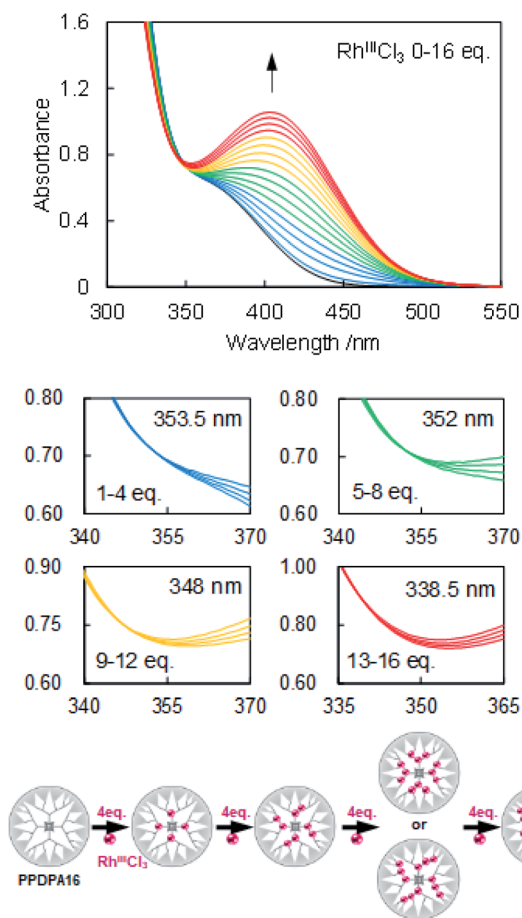
Fig. 1 Accumulation of Rh III Cl 3 to PPDPA16. (top) Change in UV-vis absorption spectra of PPDPA16 in DCM upon adding Rh III Cl 3 in MeCN/MeOH = 250/1 up to 16 eq. ([PPDPA16] = ca. 5 μM, 20 °C). (down) Enlarged views during complexation with Rh III Cl 3 in respective positions 0–4, 5–8, 9–12, and 13–16 eq. and the schematic illustration of the possible coordination sequence.
