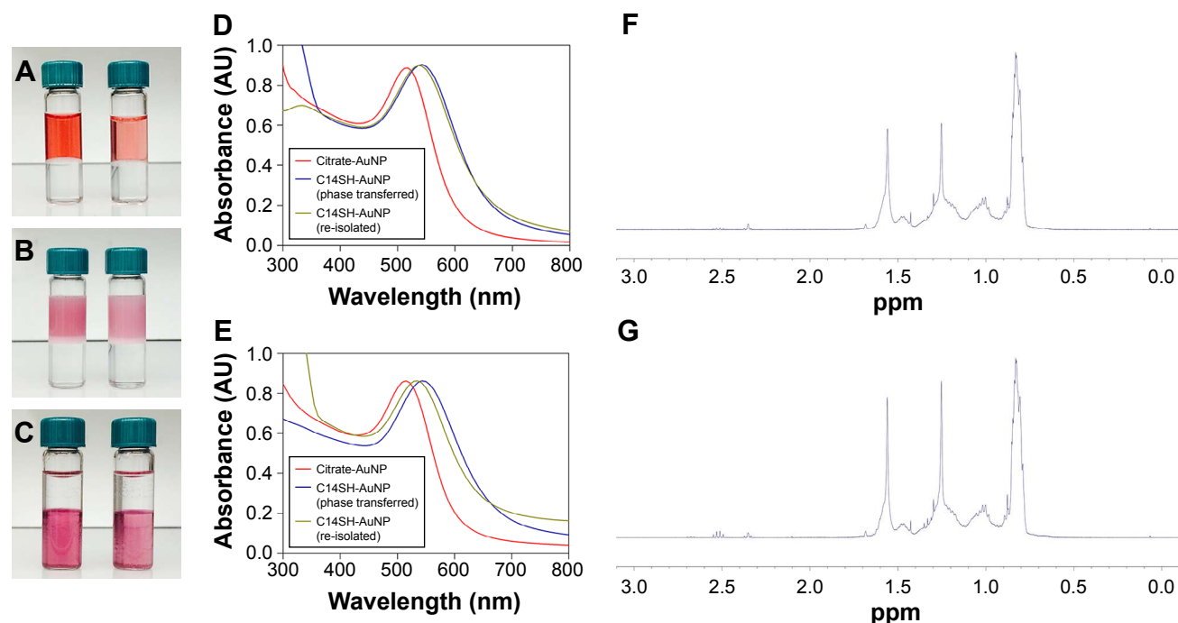
Figure 1 Preparation and spectroscopic characterization of 10 and 17 nm AuNPs. Digital photographs of AuNPs ( A ) prior to transfer, ( B ) activated by acetone/Tween 20/C14SH, ( C ) after transfer. The top and bottom layers represent the aqueous and chloroform layers, respectively. UV-Vis spectra of ( D ) 10 nm and ( E ) 17 nm AuNPs showing the particles in citrate-stabilized state, immediately after phase transfer, and upon re-isolation. ^1\text{H} NMR spectra of purified ( F ) 10 nm and ( G ) 17 nm AuNPs in \text{CDCl}_3 . The signal at 1.6 ppm corresponds to water.
