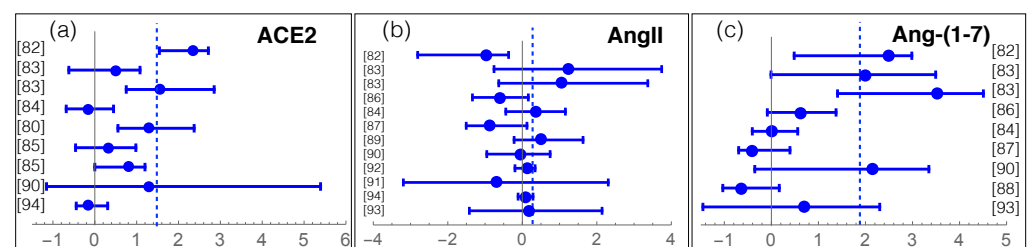
Figure 3. Log-ratios between RAS components (ACE2, AngII and Ang-(1-7)) in COVID-19 patients and controls, with the estimated confidence intervals, for all the collected studies referenced by their reference number (see Table S1). The dashed lines represent the averages of the log-ratios weighted according to the number of patients analyzed in each study. On the y-axis, the reference to the study is mentioned.
