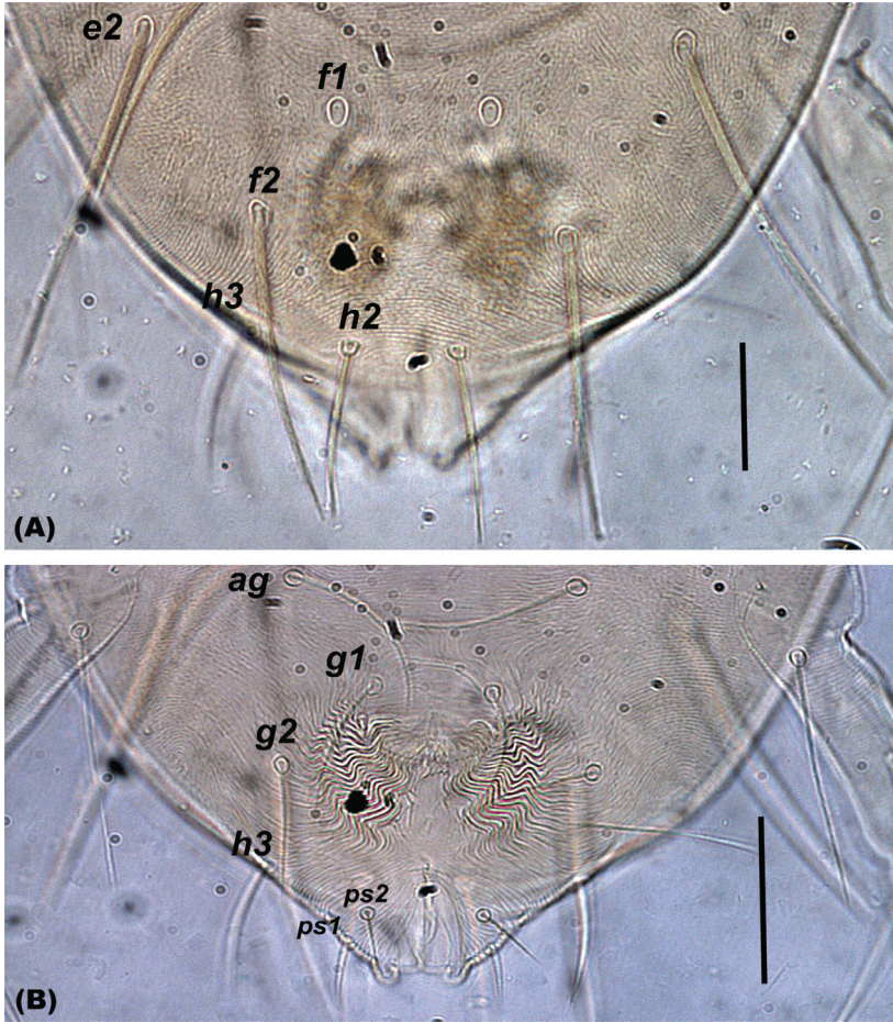
Figure 2. Shape of setae A h_2 and B h_3 are similar to other ventral body setae in all the genera of the tribe Tetranychini in e.g. Oligonychus . Scale bar: 30 \mu\text{m} .
