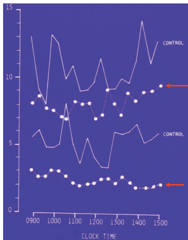
Figure 6. Spontaneous circadian LH secretion (mU/ml) in a 26 yr old TD \beta -thal patient who developed a progressive apulsatility (dotted line) of gonadotropins (De Sanctis V, personal observation)
