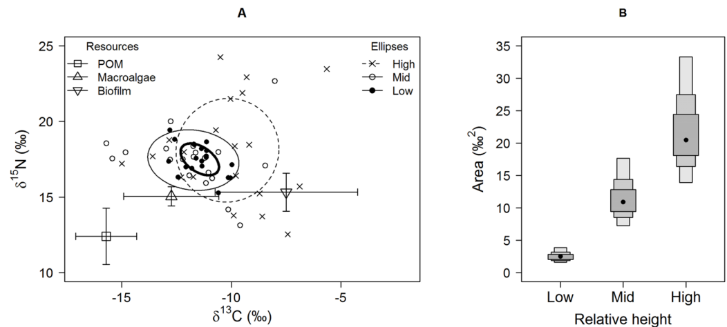
Figure 1 Isotopic variation among Echinolittorina peruviana individuals grouped by relative height on the shore. (A) Individual values on an \delta^{15}\text{N} - \delta^{13}\text{C} biplot, with standard ellipses (equivalent to a bivariate SD), corrected for small sample size (SEAc), plotted as calculated by the SIBER procedure (Jackson et al. , 2011). Plot lines and symbols represent shore height (see legend). (B) E. peruviana isotopic niche width (SEA.B) at different shore heights, plotted with 95, 75 and 50% credible intervals and mode as a black point. Macroalgae includes Lessonia nigrescens , Dictyota sp. and Ulva sp. pooled.
