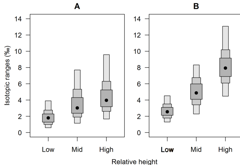
Figure 2 Separate (A) carbon and (B) nitrogen isotopic variation of E. peruviana individuals from different shore heights. Range estimates calculated by a Bayesian implementation of Layman et al. (2007) in the R package SIBER (Jackson et al. , 2011). A black dot shows the mode, while boxes represent the 95, 75 and 50% credible intervals.
