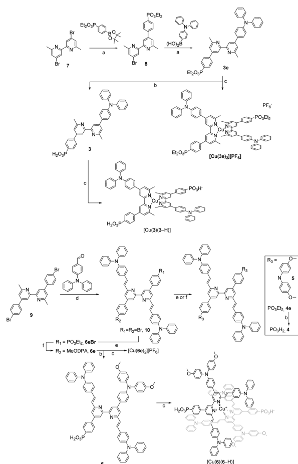
Scheme 3 Synthetic routes to ligands and homoleptic copper(I) complexes. (a) Pd(PPh 3 ) 4 , Na 2 CO 3 , Tol/H 2 O 9 : 1, 80 °C, on.; (b) TMSBr, CH 2 Cl 2 , rt, 3–24 h; (c) [\text{Cu}(\text{CH}_3\text{CN})_4][\text{PF}_6] , MeOH or CH 2 Cl 2 or CH 2 Cl 2 /MeOH 4 : 1 or CH 2 Cl 2 /CH 3 CN 1 : 1, rt, 1–18 h; (d) TMSCl, DMF, 170 °C, 48 h; (e) Pd(dppf)Cl 2 , Cs 2 CO 3 , Et 2 HPO 3 , toluene, 110 °C, 15–18 h; (f) Pd(dba) 2 , RuPhos, t BuONa, 15–18 h, THF or toluene, 90 °C.
