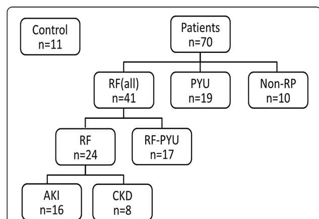
Figure 1 Schematic illustration of the case groupings used in this study. A total of 81 samples were analyzed. Based on the patients' clinical parameters, the samples were classified into a number of different groups. These were the RF group with azotemia, the RF-PYU group with azotemia and pyuria, the PYU group with pyuria but without azotemia, the non-RP group with diseases unrelated to azotemia and pyuria; the AKI groups with acute kidney disease and the CKD group with chronic kidney disease.
