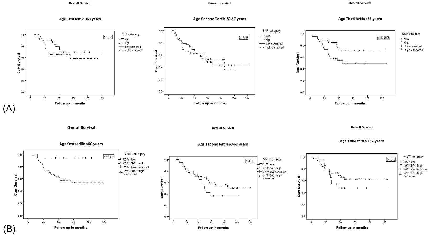
Fig. 4. Kaplan–Meier curves of the effects on overall survival of the VNTR and SNP categories stratified to age tertiles. (A) SNP category; (B) VNTR category.
