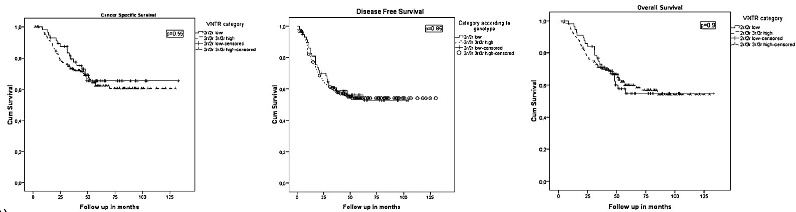
Fig. 3. Kaplan-Meier schemas for OS, DFS and CSS according to (A) SNP categories TS low (2R homozygous plus C allele) and high (G allele) producers (B) VNTR categories (2R/2R low vs. 2R/3R and 3R/3R high).
