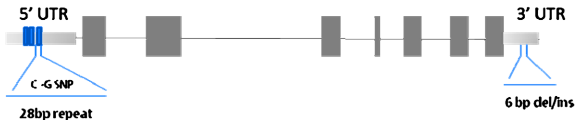
Fig. 1. Schematic representation of the TYMS gene with known polymorphisms in 5' untranslated region (5'-UTR) and 3'-UTR. On the 5'-UTR the 28 bp repeat with the SNP in the third repeat. On the 3'-UTR a 6 bp long deletion/insertion.
