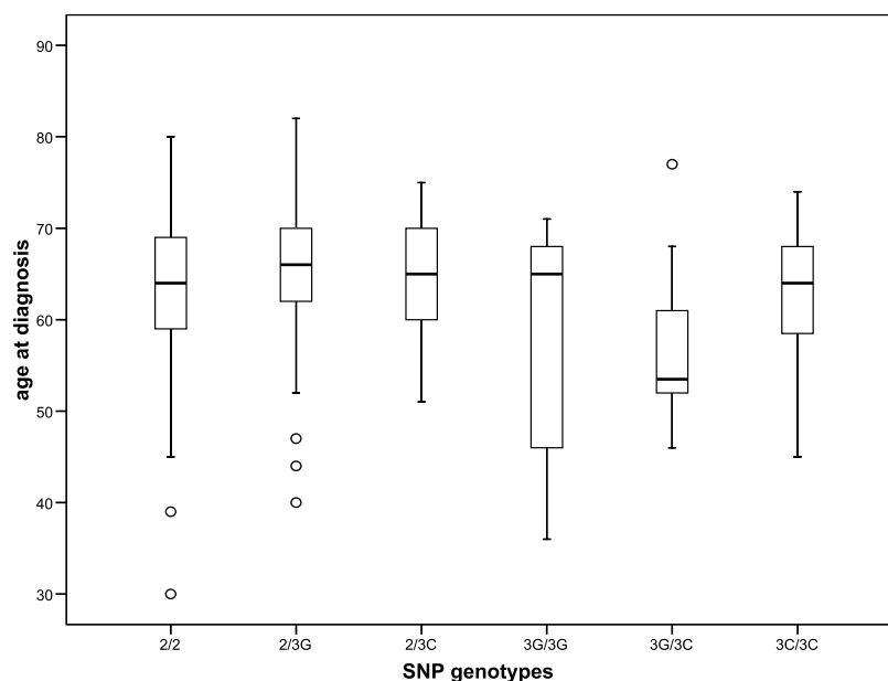
Fig. 2. Age distribution according to SNP genotypes (Kruskal–Wallis H = 15.135 , p = 0.01 , 99% CI 0.006–0.0).
