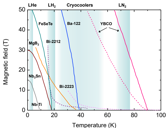
Figure 3. Comparative H - T phase diagram for representative cuprates, iron-based superconductors, MgB_2 and conventional superconductors
