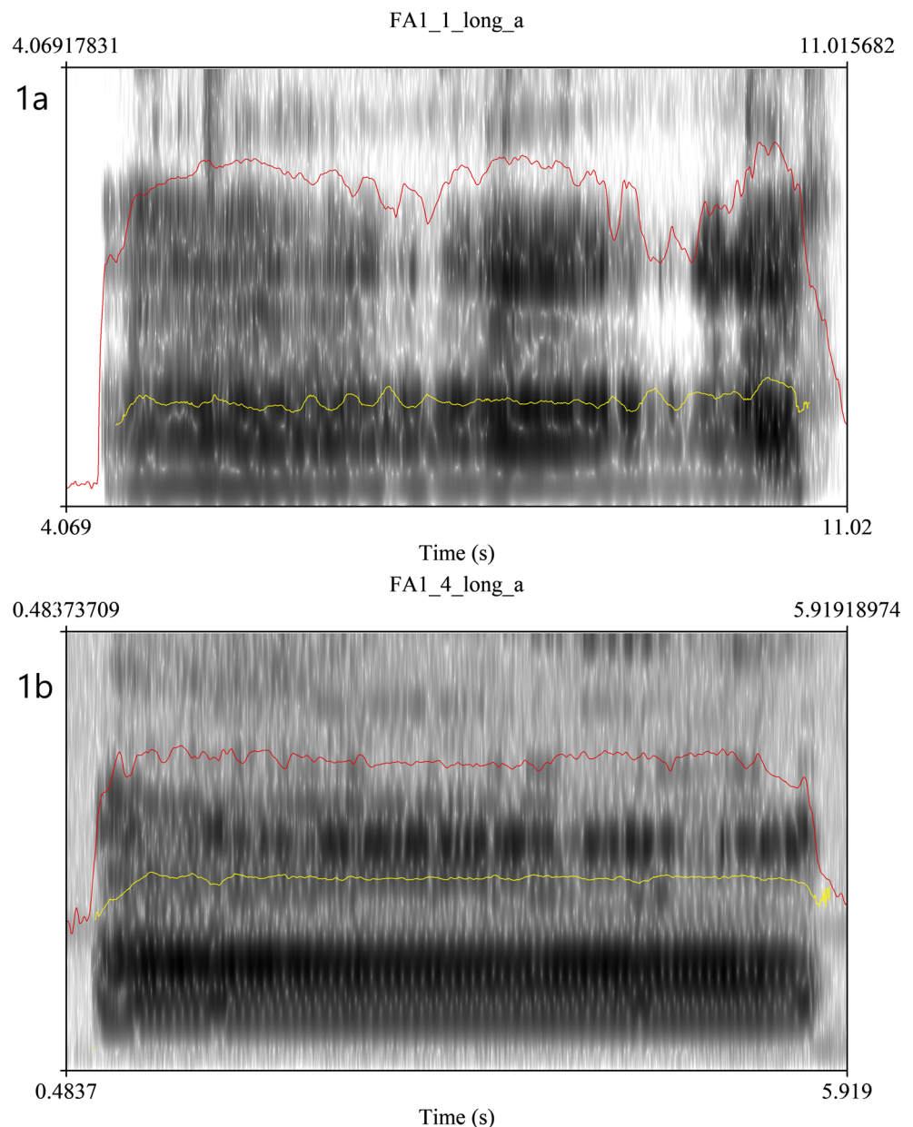
Fig. 1 Oscillogram and spectrogram plots of prolonged vowel for session 1 (a) and session 4 (b) for participant 1. The red line represents the loudness contour, and the yellow line the pitch contour
