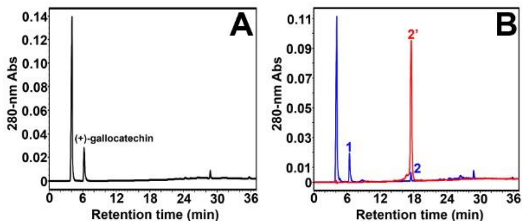
Figure 6. Reverse-phase HPLC analysis of VvANS product of (+)-gallocatechin. (A) HPLC analysis of the reaction mixture containing 100 \mu\text{M} (+)-gallocatechin without enzyme. (+)-Gallocatechin is eluted at 6.2 min, and no product is observed; (B) HPLC overlay chromatogram of the enzymatic products of (+)-catechin (in red) and the commercial standard of 100 \mu\text{M} cyanidin chloride (in blue). The blue peak 1 corresponds to (+)-gallocatechin (residual). The two large peaks observed at 4.0 min in (A) and (B) correspond to ascorbate.
