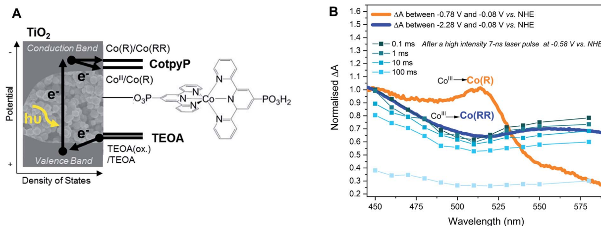
Fig. 6 Transient and steady state spectroelectrochemical characterisation of the \text{CO}_2 -reduction catalyst CotpyP on \text{TiO}_2 in ACN 0.1 M \text{TBAPF}_6 and 0.1 M TEOA. (A) Scheme of the photocatalytic system, where the arrows indicate the direction of electron transfers. (B) Comparison between photoinduced transient spectra (after \sim 1.4 \text{ mJ cm}^{-2} 355 nm excitation with 0.8 Hz laser repetition rate under -0.58 \text{ V vs. NHE} ) and electrochemically-induced steady state spectra of \text{TiO}_2 - CotpyP in ACN 0.1 M \text{TBAPF}_6 0.1 M TEOA.
