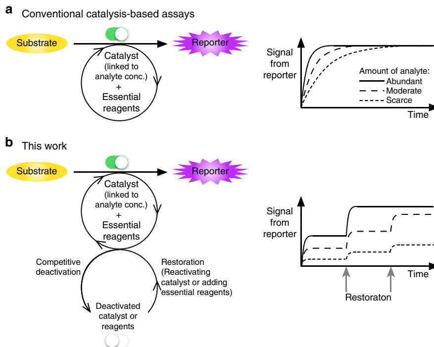
Figure 6 | Continuous reaction and competitively and reversibly deactivated reaction. (a) Widely used catalytic assays continuously convert a substrate to a reporter molecule. (b) This work presents a stop-and-go paradigm, in which there is a competition between the catalytic reaction and autonomous deactivation of the catalyst (that is, analyte) or the essential reagent. The addition of an activator or a reactant restores the system.
