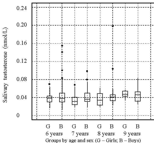
Figure 3 Box and whiskers plot for salivary testosterone levels (nmol/L) in girls and boys by age groups. The central horizontal lines within the box represent the median of the sample group. Lower and upper lines represent two quartiles of the measured value. The vertical line indicates the range of values falling within 1.5 times the interquartile. Asterisks denote values that are greater than 1.5 times the interquartile range.
