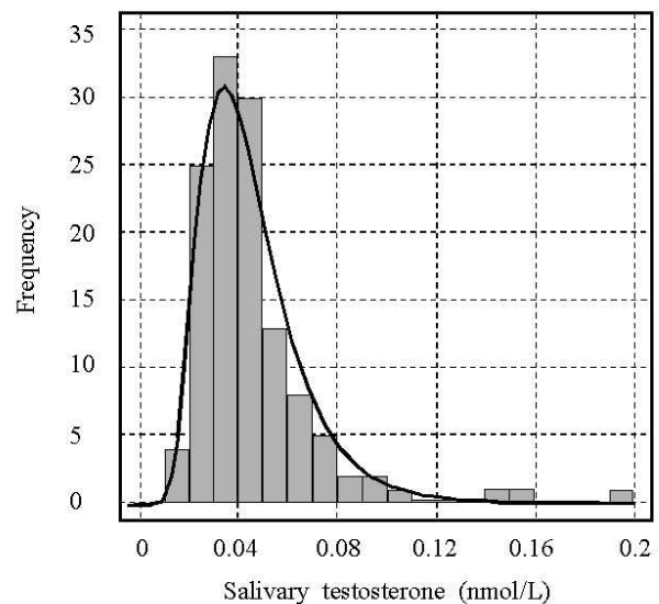
Figure 2 Lognormal distribution of salivary testosterone levels (nmol/L) in prepubertal boys.
