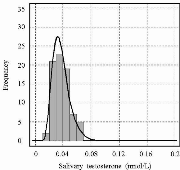
Figure 1 Lognormal distribution of salivary testosterone levels (nmol/L) in prepubertal girls.
