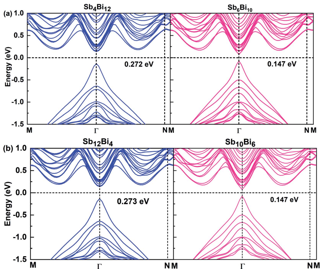
Fig. 7 Band structures of (a) \text{Sb}_4\text{Bi}_{12} LHS (left) and \text{Sb}_6\text{Bi}_{10} LHS (right), (b) \text{Sb}_{12}\text{Bi}_4 LHS (left) and \text{Sb}_{10}\text{Bi}_6 LHS (right) using PBE + SOC method.
