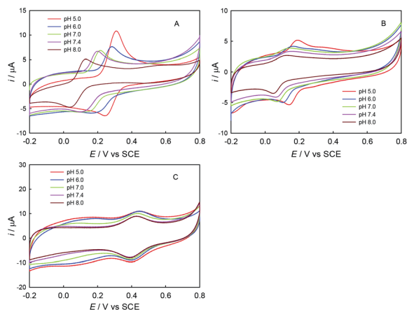
Fig. 1 CV curves on GCE in 0.1 M phosphate buffer (pH 5.0, 6.0, 7.0, 7.4, or 8.0) containing 0.1 M K_2SO_4 and 0.100 mM ChA (A), 0.100 mM trolox (B), or 0.100 mM ABTS (C). Scan rate: 100\text{ mV s}^{-1} ; initial potential: -0.2\text{ V} .
