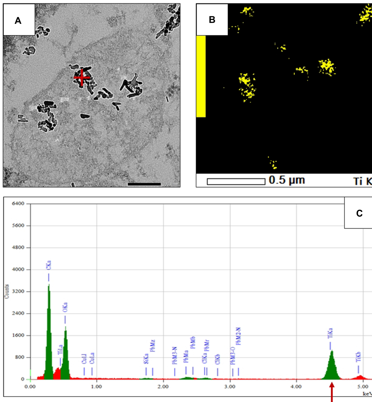
Figure 6 Presence of TiO 2 nanorods in the kidney cortical tissue of a treated rat from the medium dose (MD) group. (A) Transmission electron micrograph showing nanorods attached to a mitochondrion (25,000×, scale bar 200 nm). (B) Energy dispersive spectroscopic mapping shows presence of Ti in the nanorods visualized in (A) . (C) spectrum taken from the area marked by red cross in (A) featuring a very strong TiO 2 Kα peak (arrow). Abbreviations: Ti, titanium; TiO 2 , titanium oxide.
